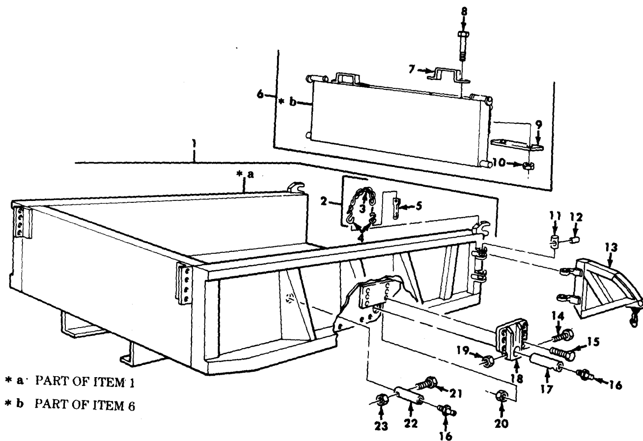
Figure 307. Dump Body, Basic, Tailgate, and Related Parts.
