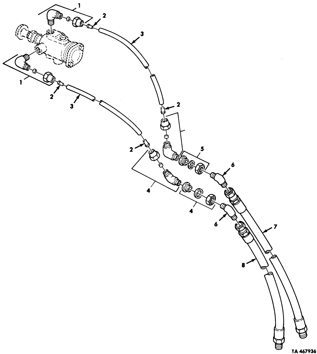
Figure 204. Dash Control Air Supply Lines, Spring Brake Control Valve to Primary and Secondary Air Reservoirs.
