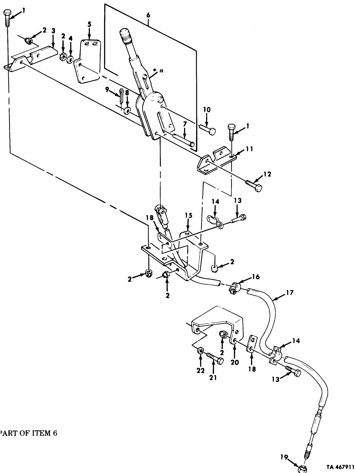
Figure 178. Parking Brake Lever Assembly, Cable, and Mounting Hardware.
