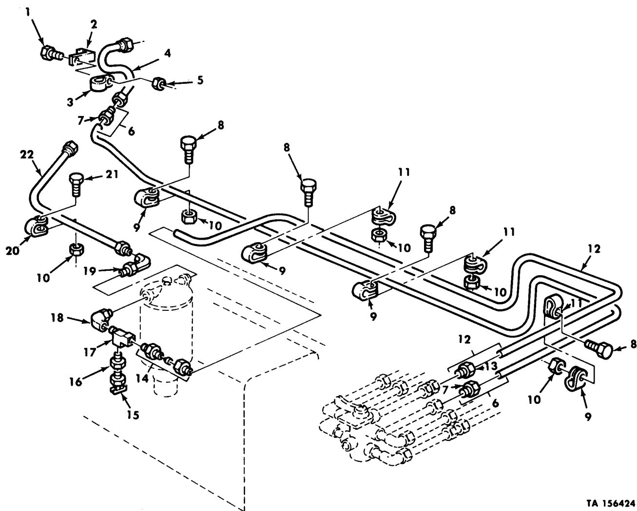
Figure 46. Fuel Tank Supply and Return Lines, Dual.
