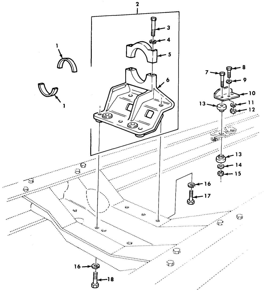
Figure 2. Engine Mounts.
