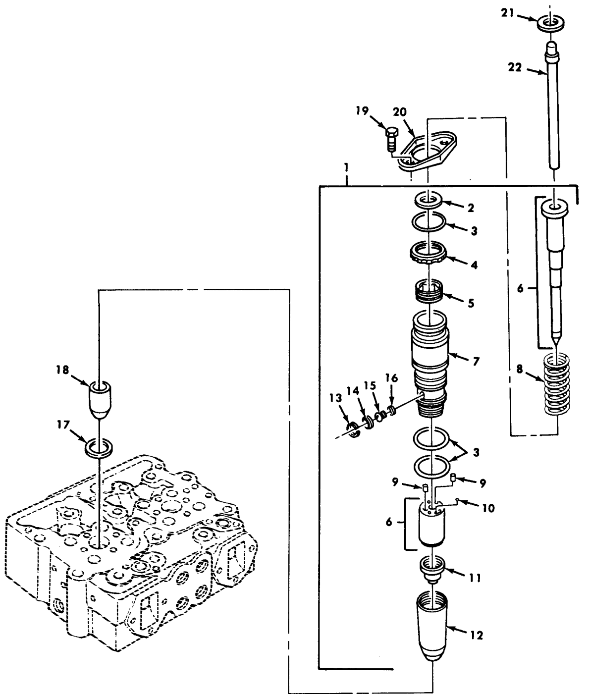
Figure 27. Fuel Injector Assembly and Related Parts.
