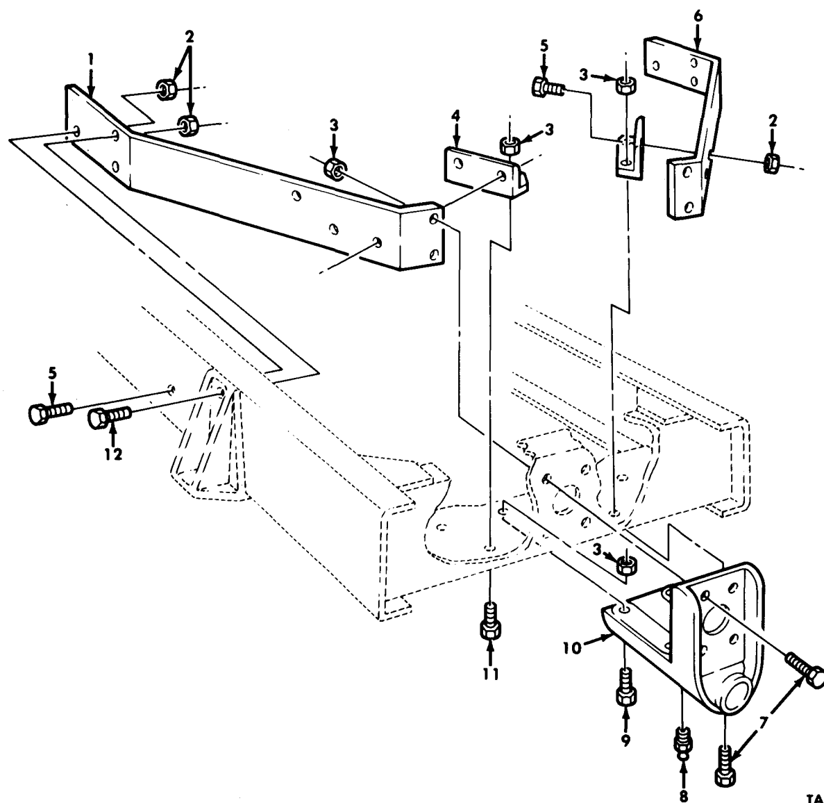
Figure 250. Towing Pintle Mounting Brackets, Tractor.
