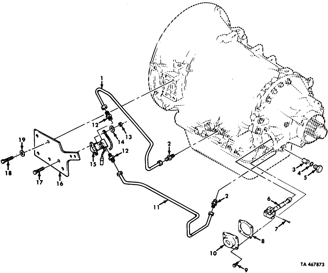
Figure 137. Transmission Tubing, Governor, and Filter Assembly.
