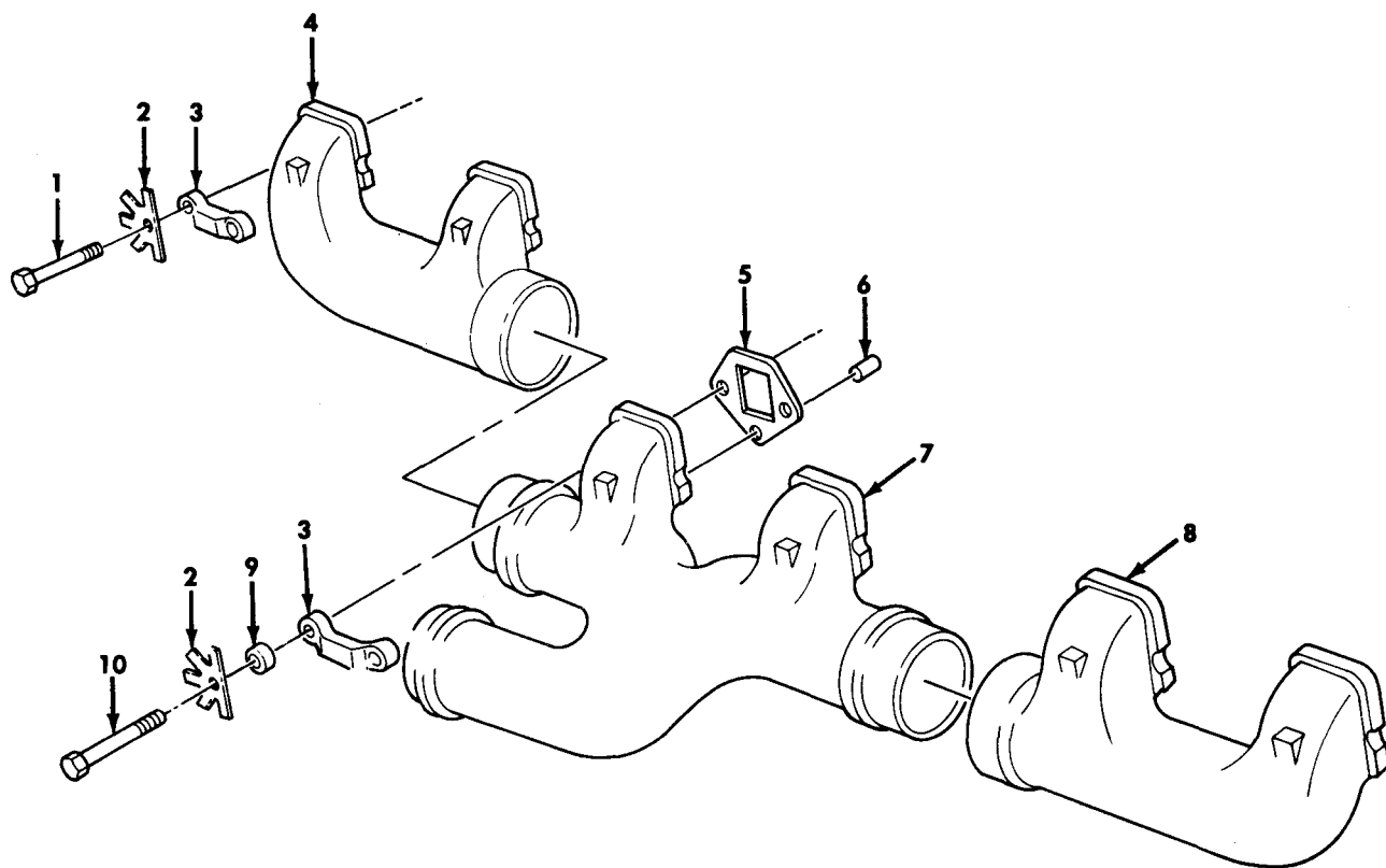
Figure 25. Exhaust Manifold.
