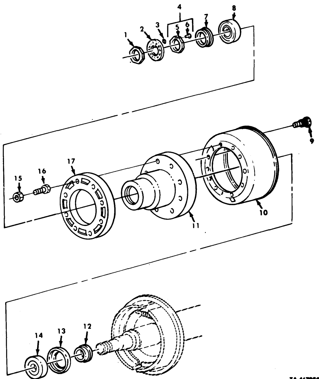
Figure 225. Rear Wheel Hub and Drum Assembly.
