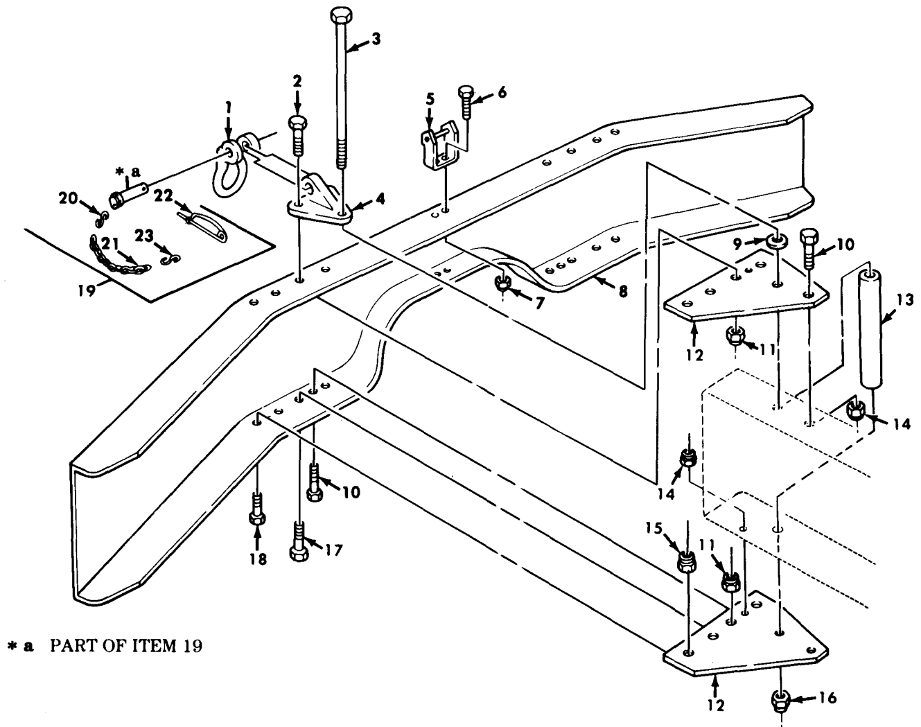
Figure 246. Front Bumper, Lifting Shackle, Hood Latch, and Mounting Hardware.
