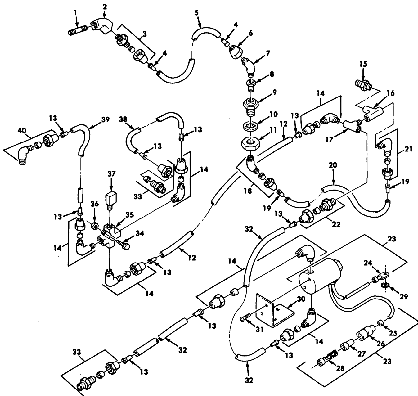
Figure 149. Transfer Air-Actuated Controls and Interlock Valve.
