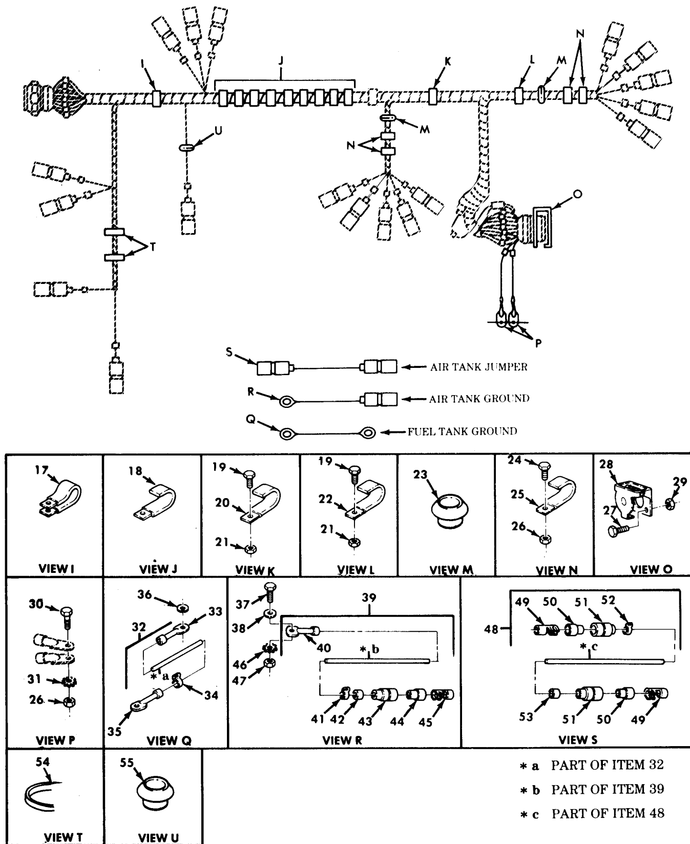
Figure 110. Rear Wiring Harness Assembly, Cargo (Sheet 2 of 2).
