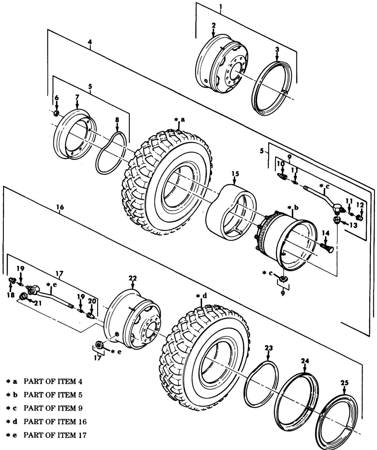
Figure 223. Wheel Assembly, Wheel and Beadlock.
