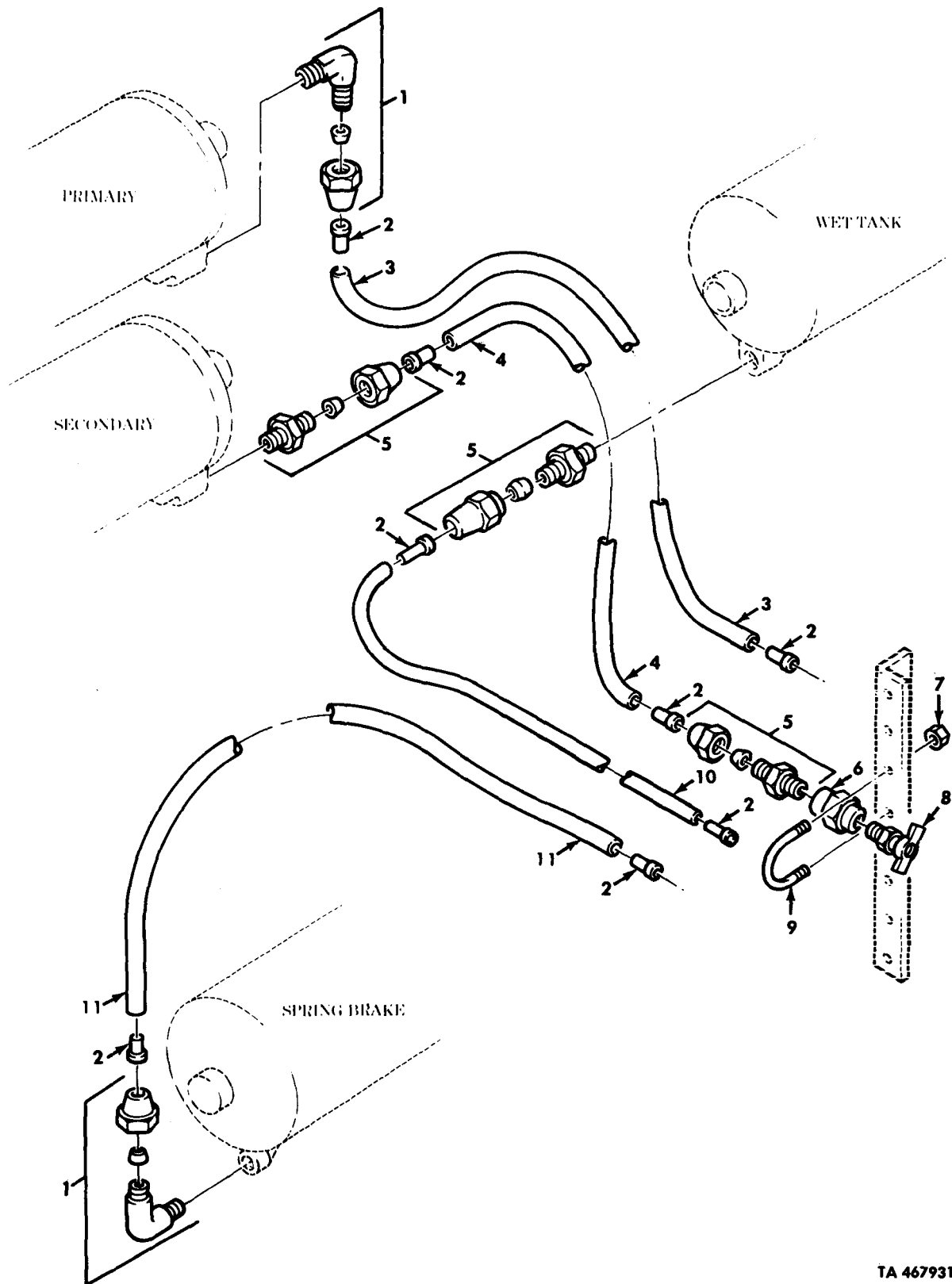
Figure 199. Air Tank Reservoir, Draincocks, and Related Lines.
