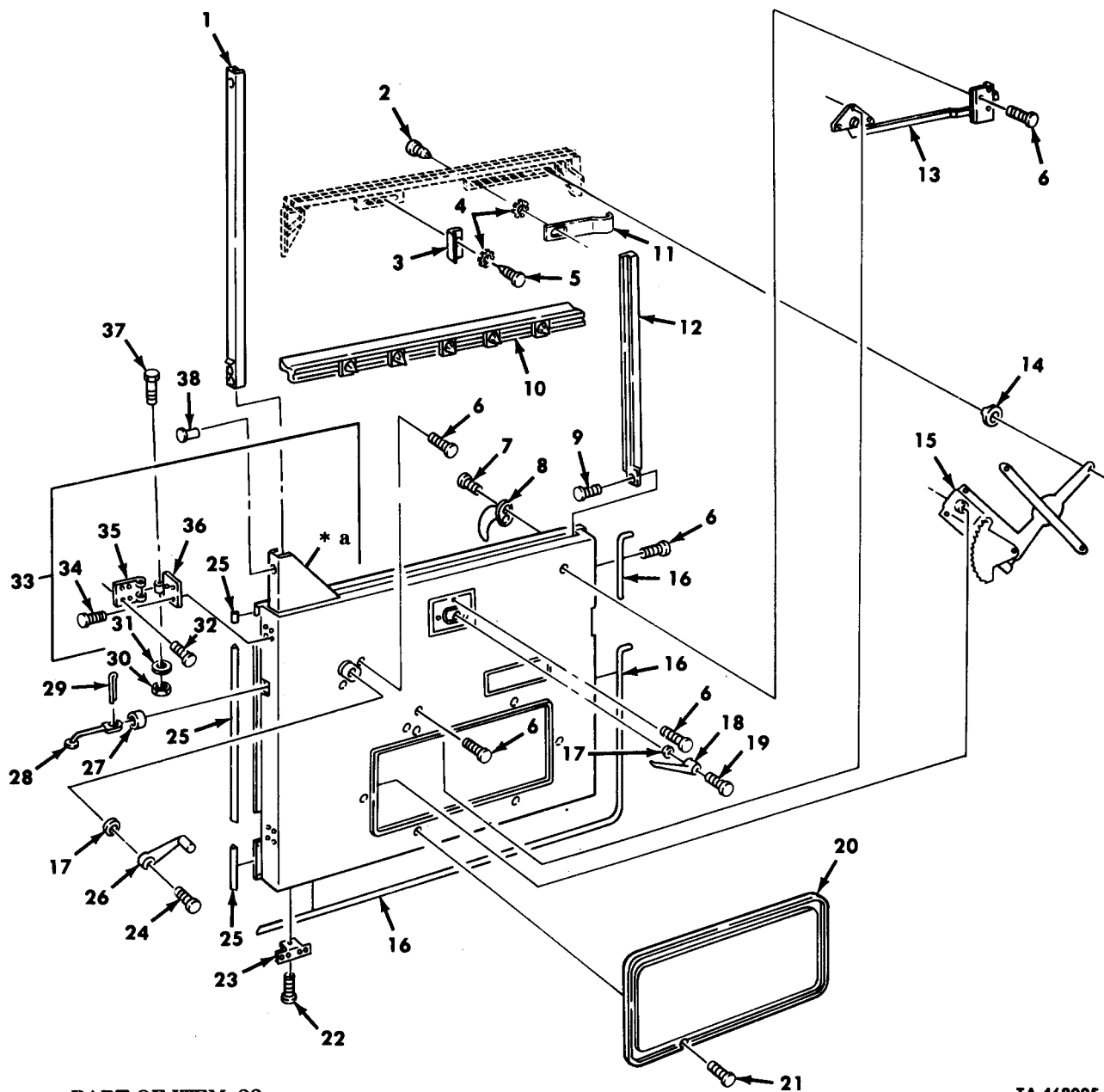
Figure 280. Door, Cab Assembly.
