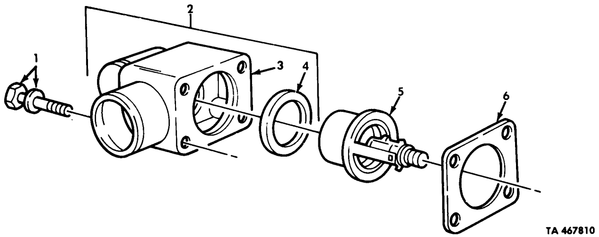
Figure 73. Thermostat, Housing, Seal, and Mounting Hardware.
