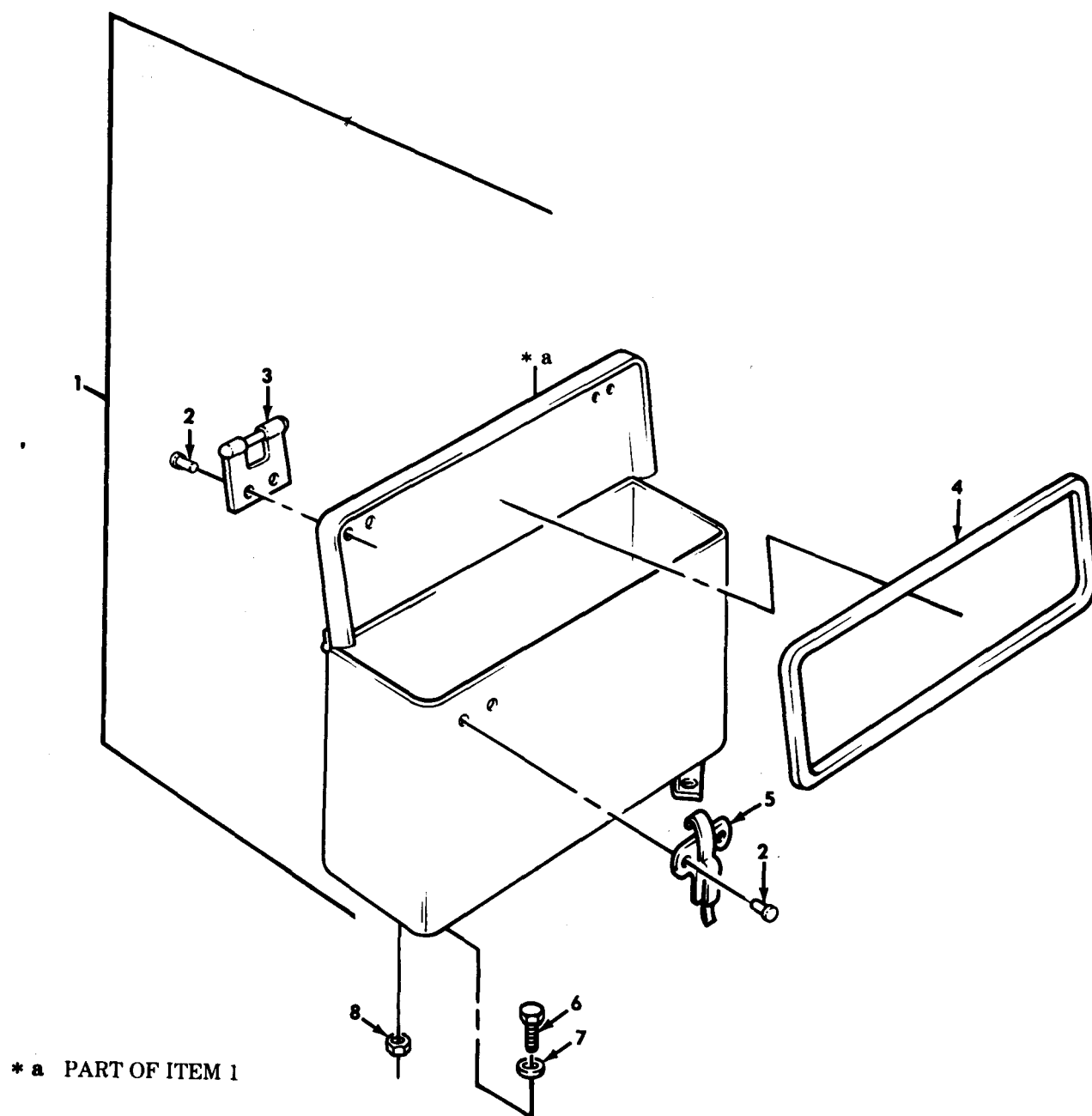
Figure 292. Map Compartment and Mounting Hardware.
