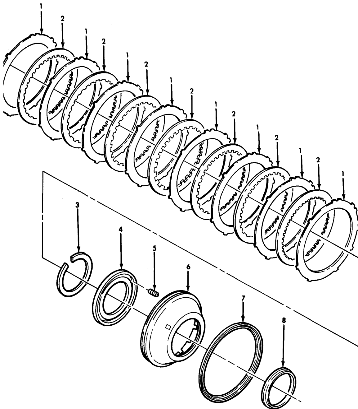
Figure 133. Low Clutch.
