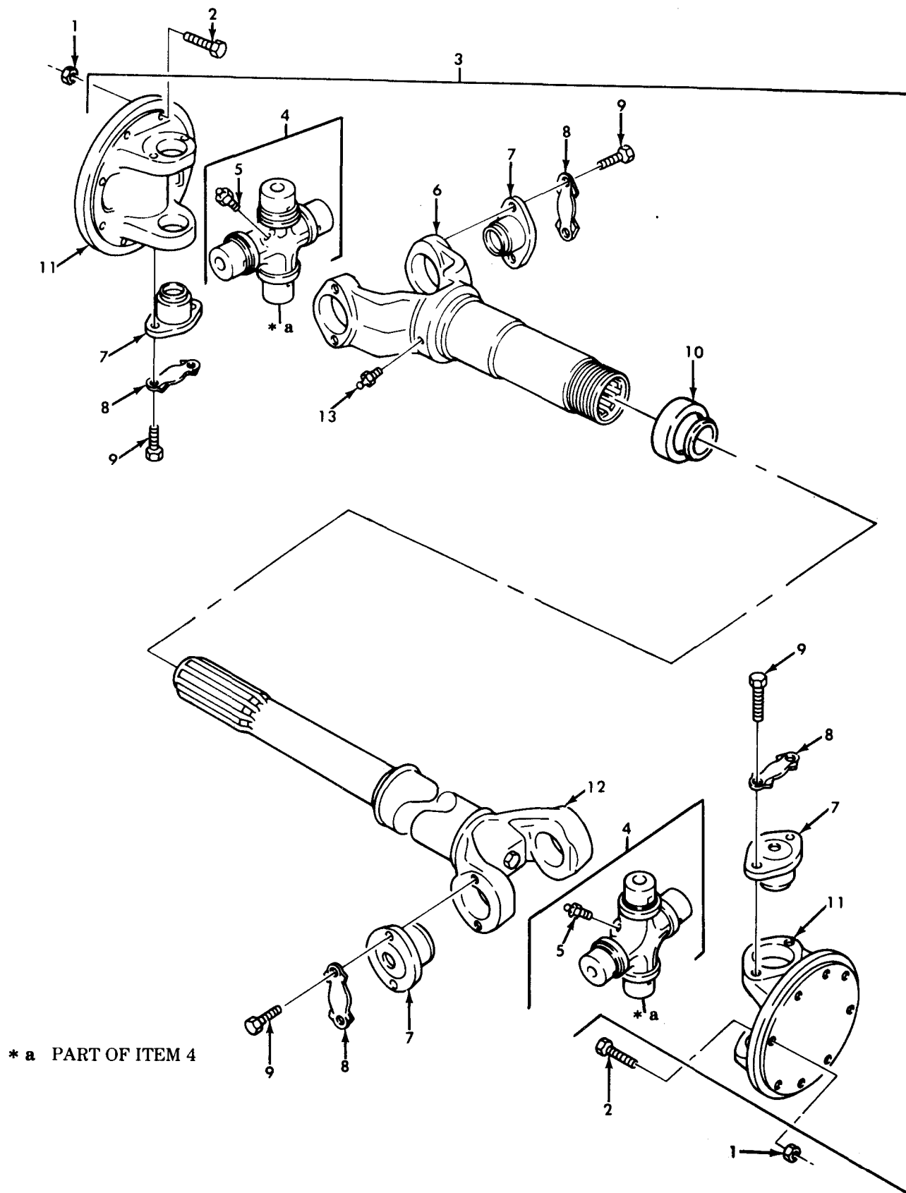
Figure 164. Propeller Shaft Assembly, Forward Rear Axle to Rear Rear Axle.
