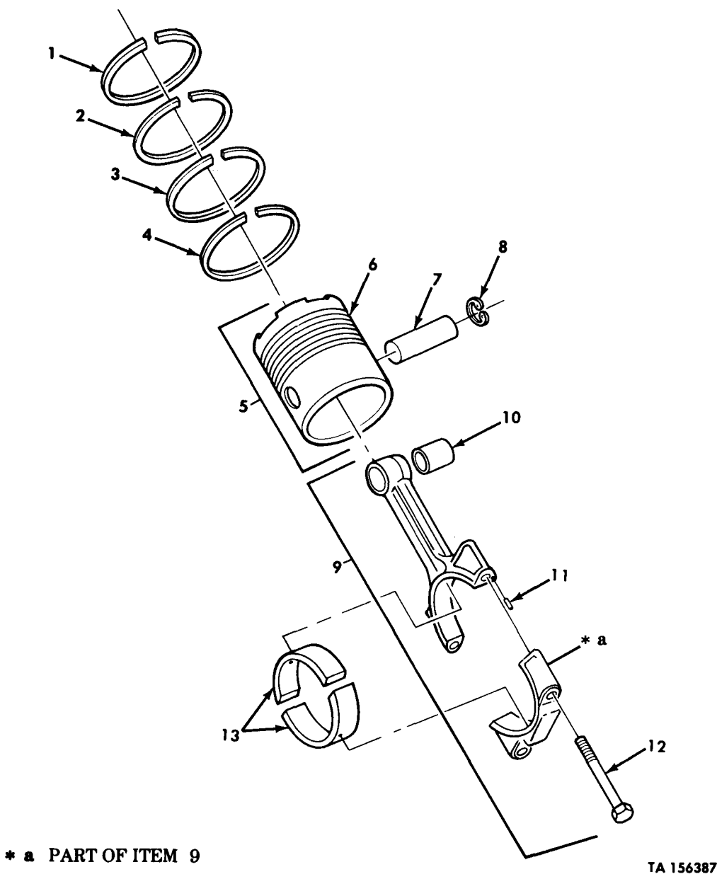
Figure 10. Piston and Rod Assemblies.
