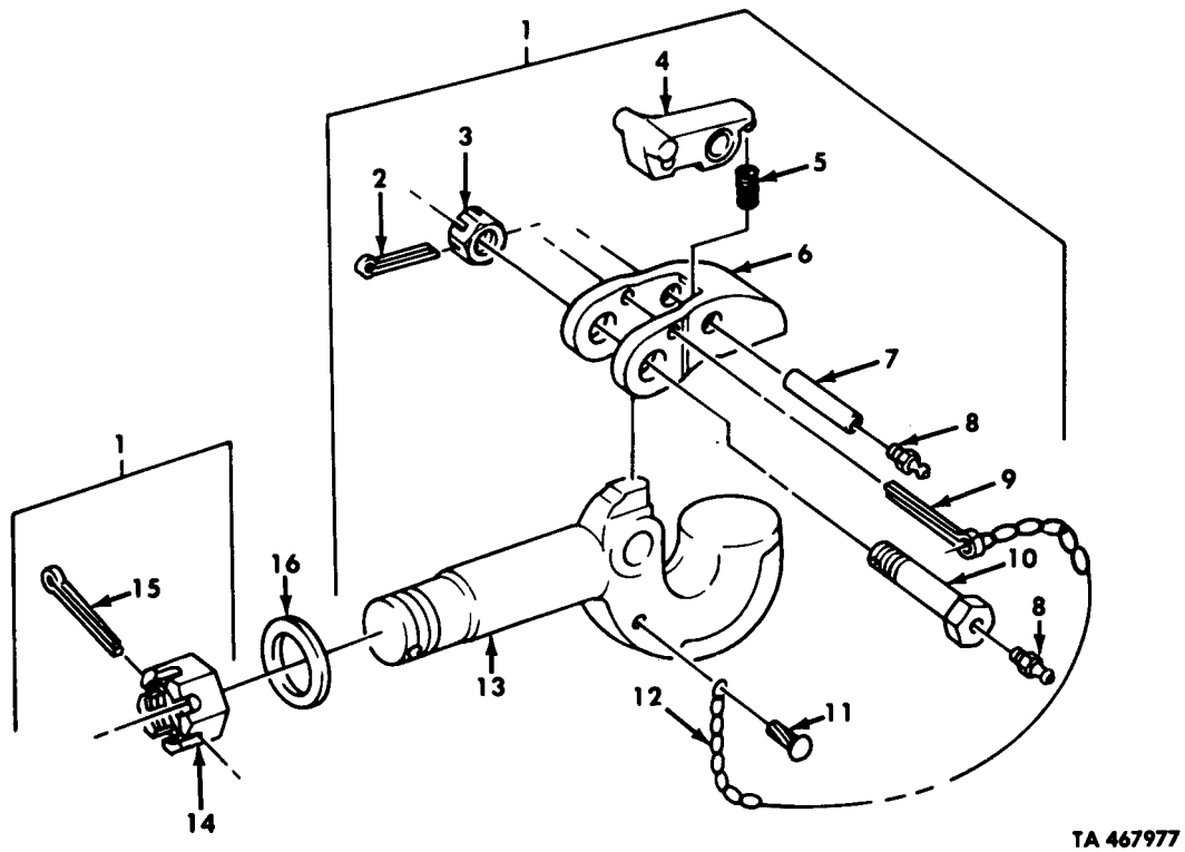
Figure 249. Pintle Hook Assembly.
