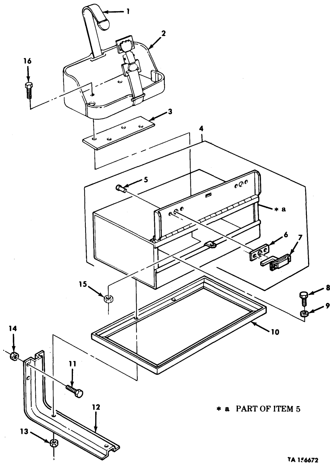
Figure 293. Toolbox Fuel Can Bracket and Mounting Hardware,
