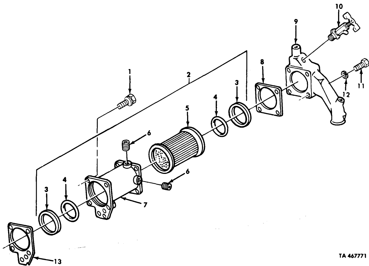
Figure 23. Engine Oil Cooler Assembly.
