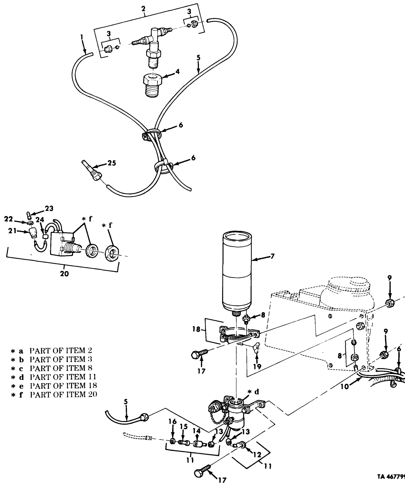
Figure 62. Ether Start Cylinder, Switch, and Related Lines and Fittings.
