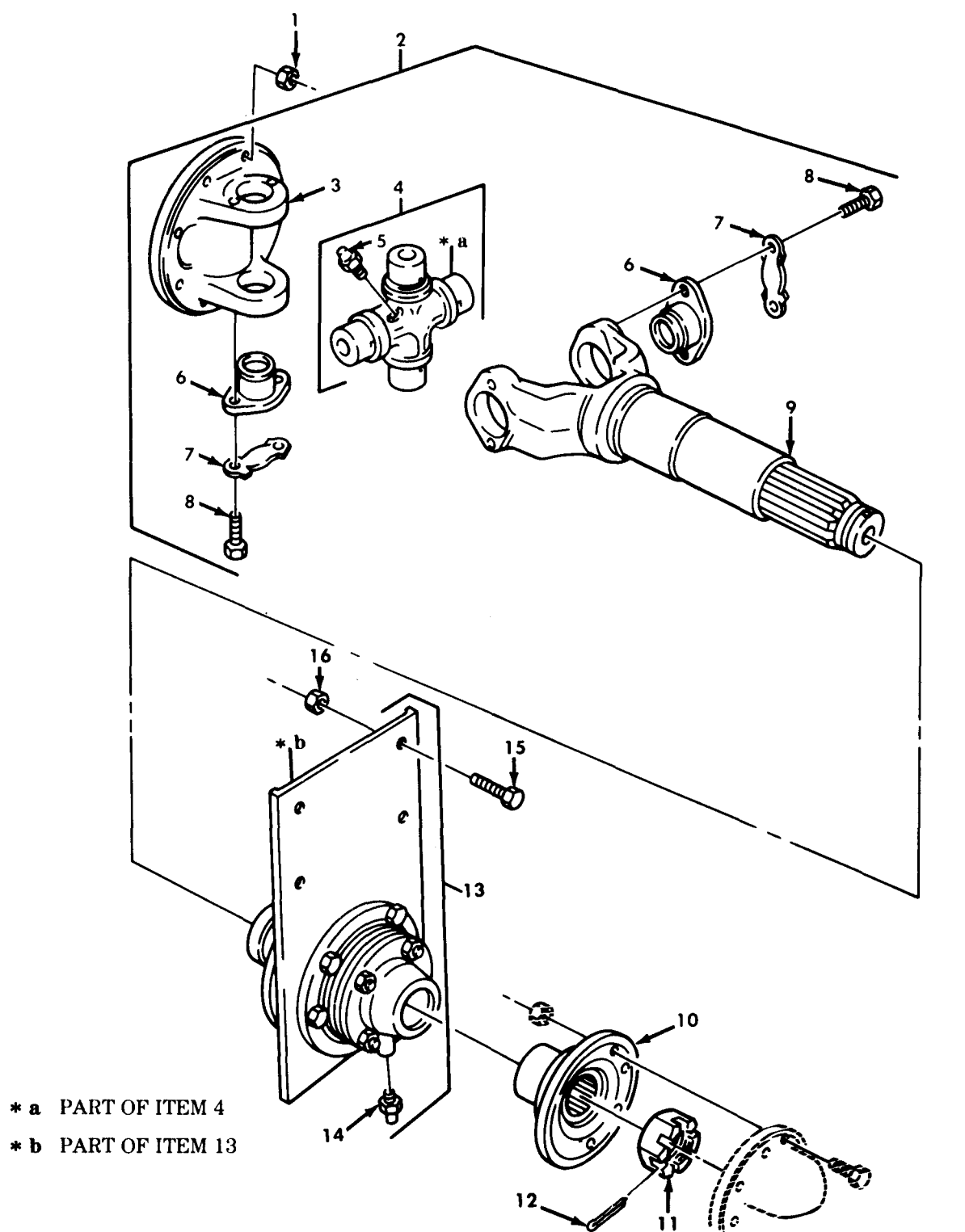
Figure 159. Propeller Shaft Assembly, Transfer to Center Bearing and Center Bearing Assembly.
