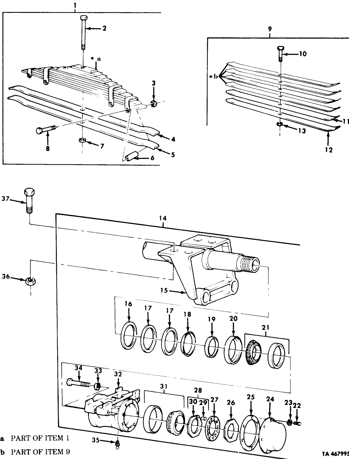
Figure 268. Rear Leaf Spring and Seat Assemblies.
