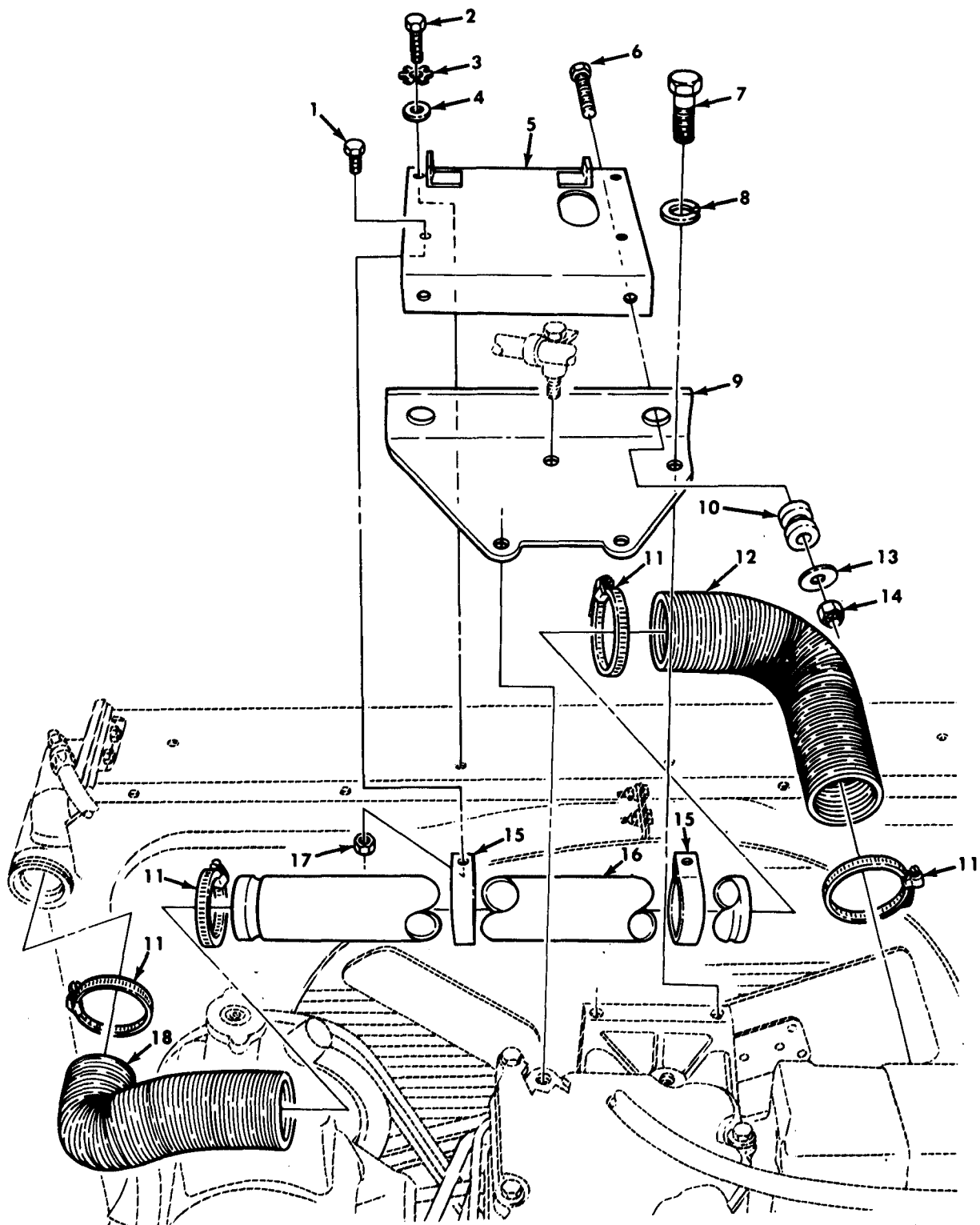
Figure 68. Upper Radiator Mounting and Hoses.
