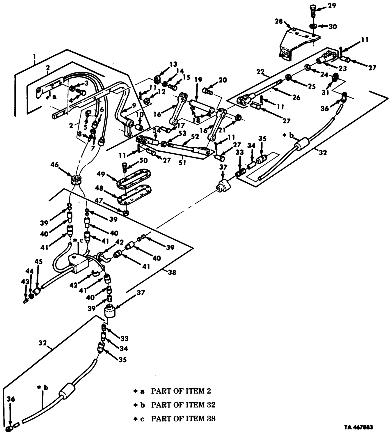
Figure 147. Transfer Controls.
