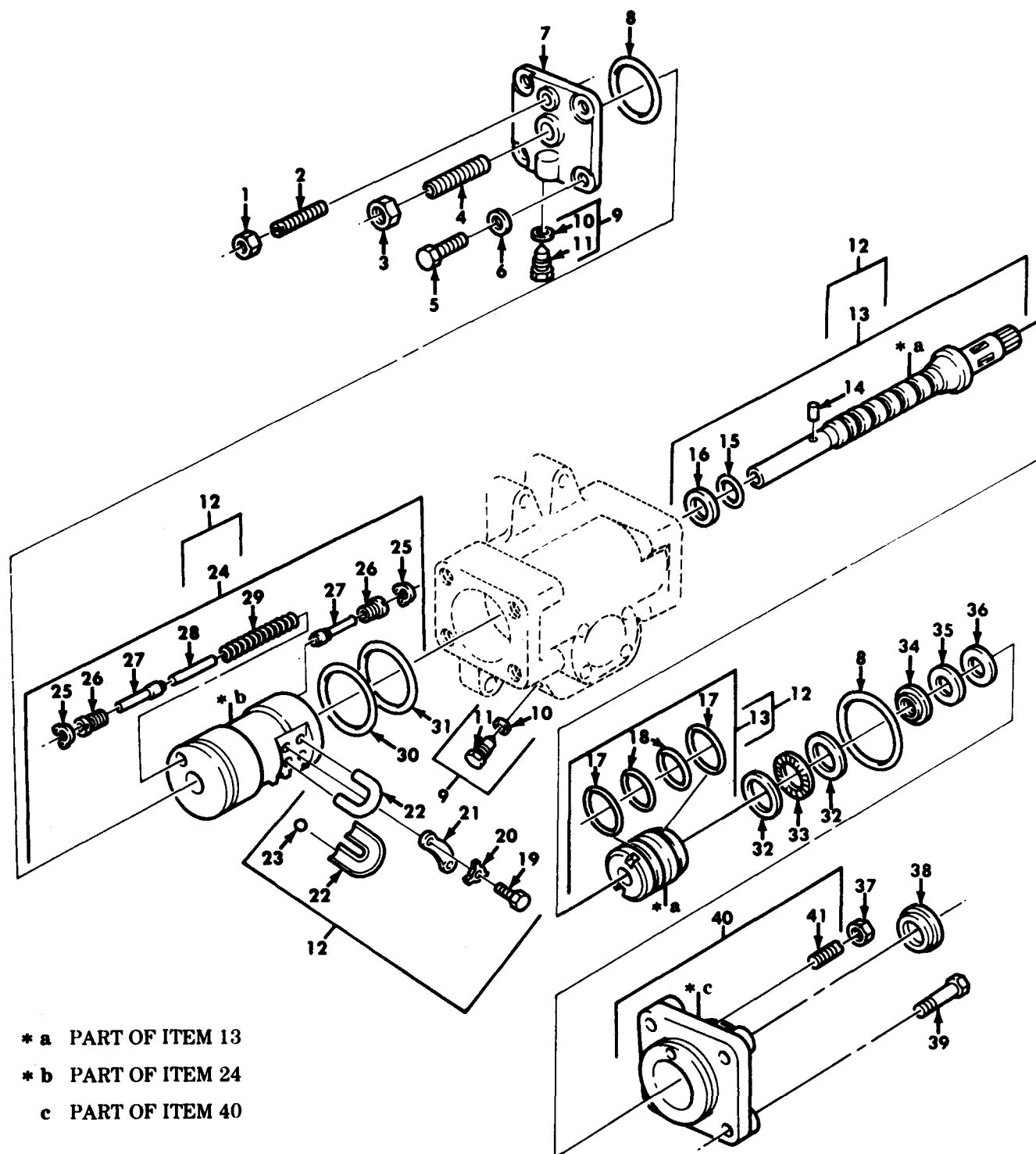
Figure 232. Steering Gear, Worm, Valve, and Rack Assembly.
