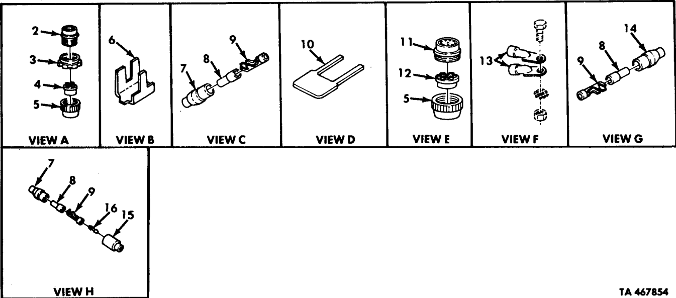
Figure 116. Rear Wiring Harness Assembly, Chassis (Sheet 1 of 2).
