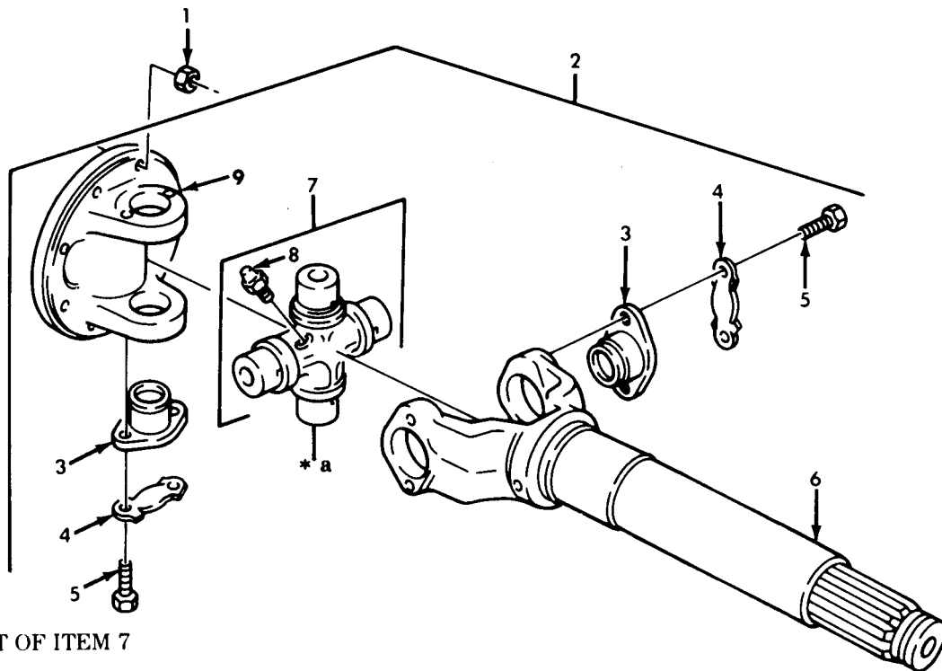
Figure 165. Propeller Shaft Assembly, Transfer to Center Bearing.
