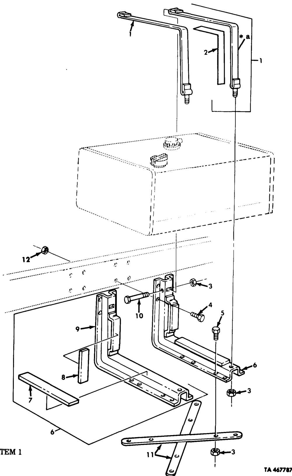
Figure 40. Fuel Tank Mounting, Single Tank, R.H.
