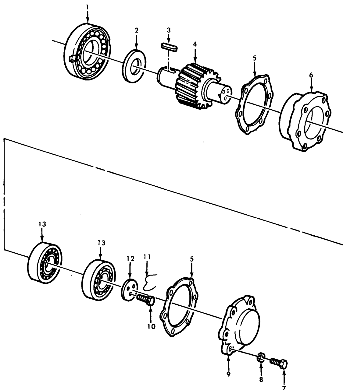
Figure 177. Rear Axle Differential Helical Drive Pinion and Related Parts.
