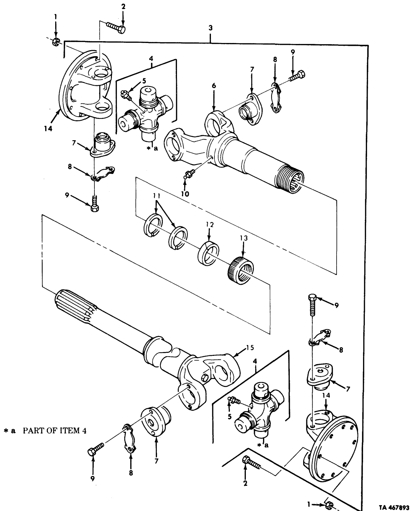
Figure 160. Propeller Shaft Assembly, Center Bearing to Forward Rear Axle.
