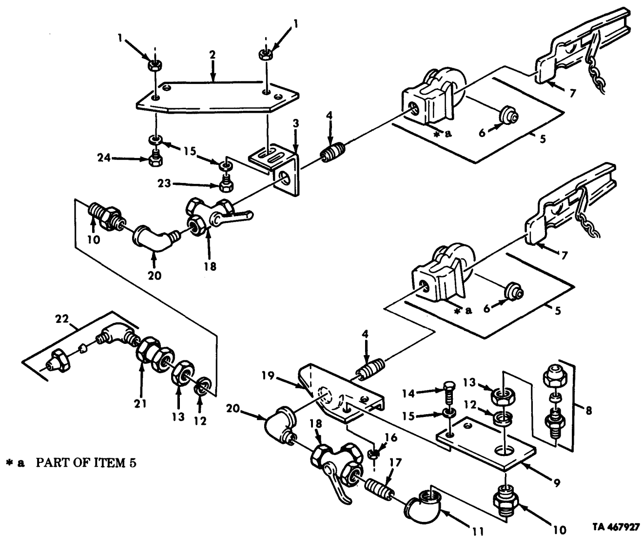
Figure 196. Rear Emergency Half Couplings and Mounting Hardware.
