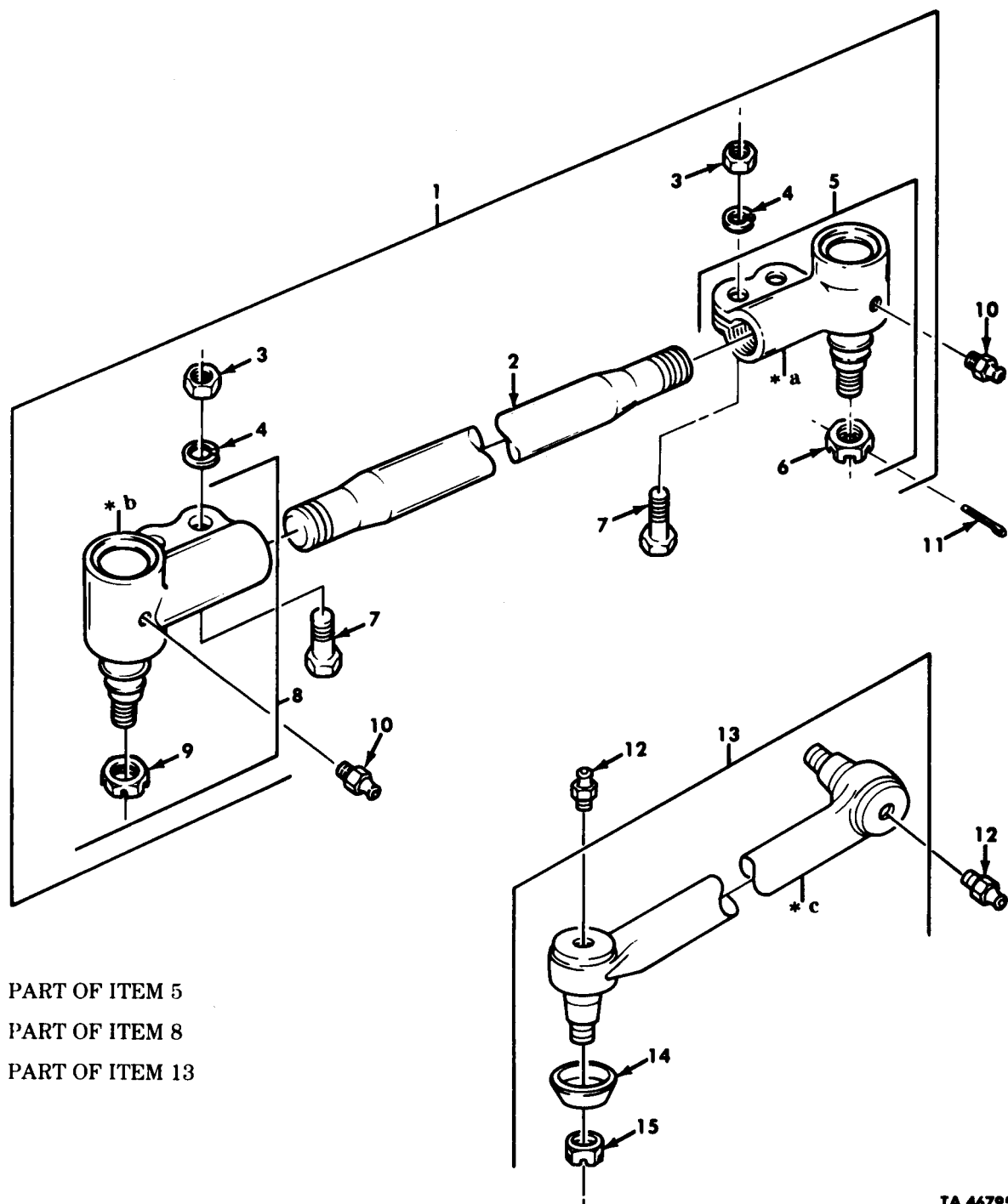
Figure 229. Tie Rod Assemblies.
