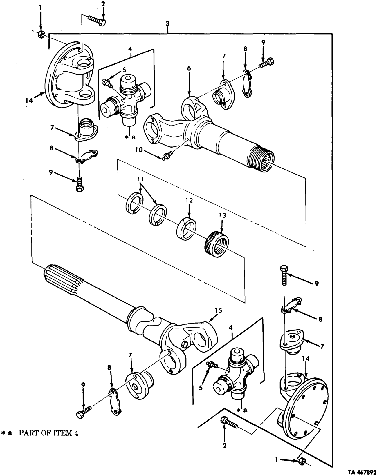
Figure 158. Propeller Shaft Assembly, Forward Rear Axle to Rear Rear Axle.
