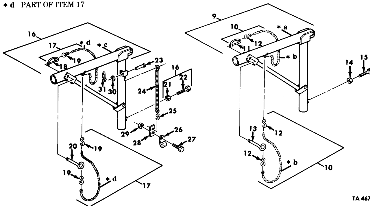
Figure 259. Lifting Device and Davit Assemblies.
