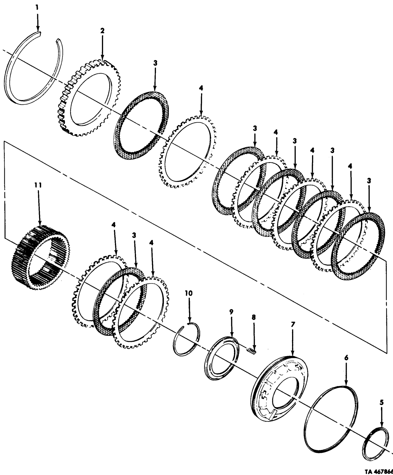
Figure 131. First Clutch.
