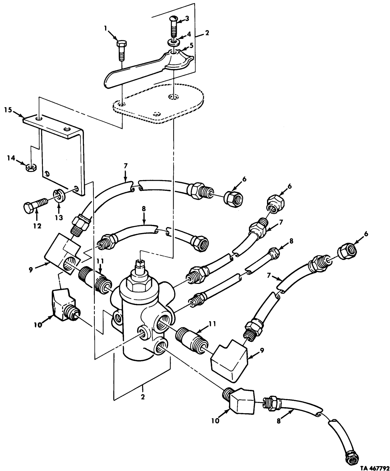
Figure 51. Fuel Tank Selector Valve Assembly and Related Parts.
