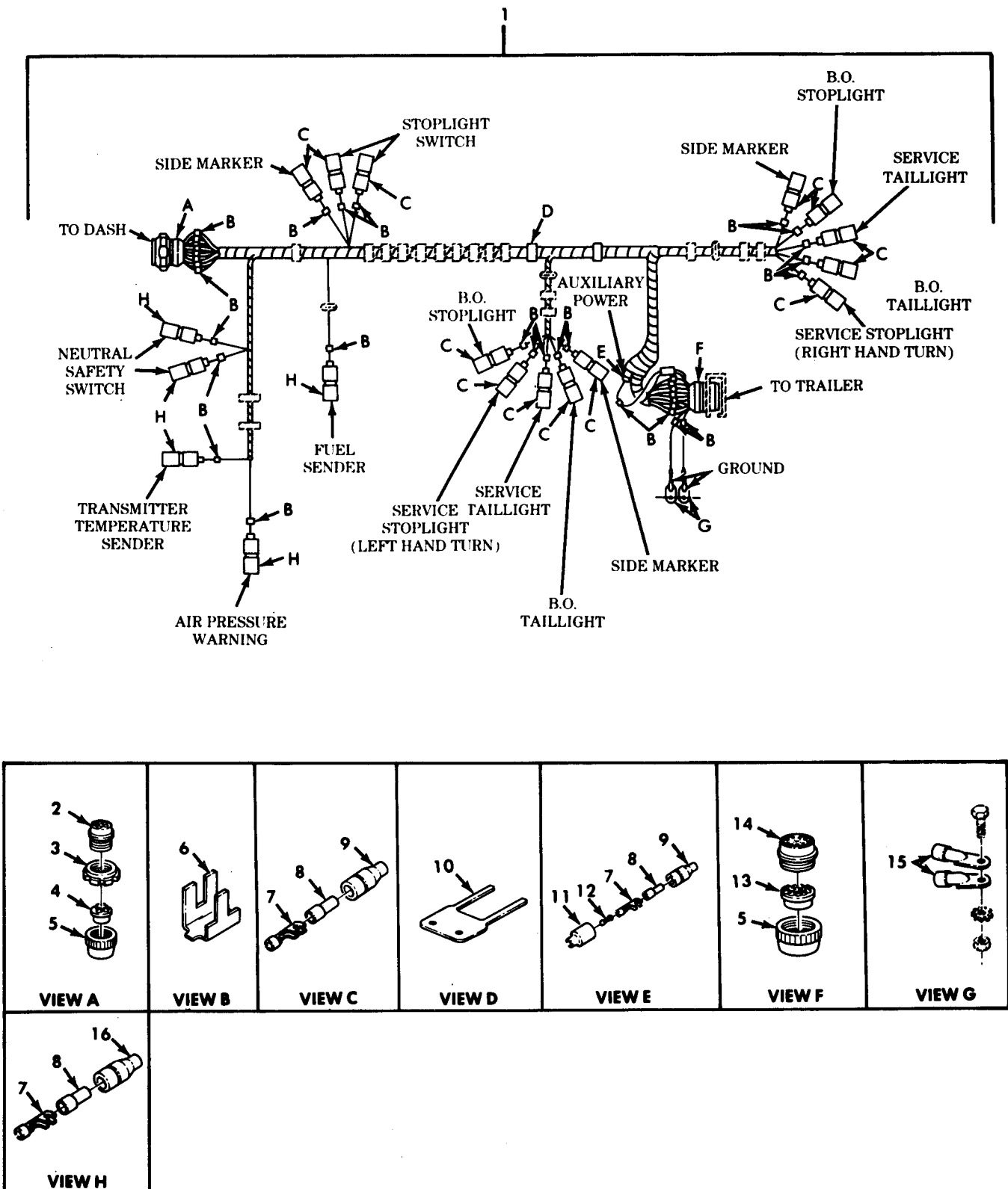
Figure 110. Rear Wiring Harness Assembly, Cargo (Sheet 1 of 2).
