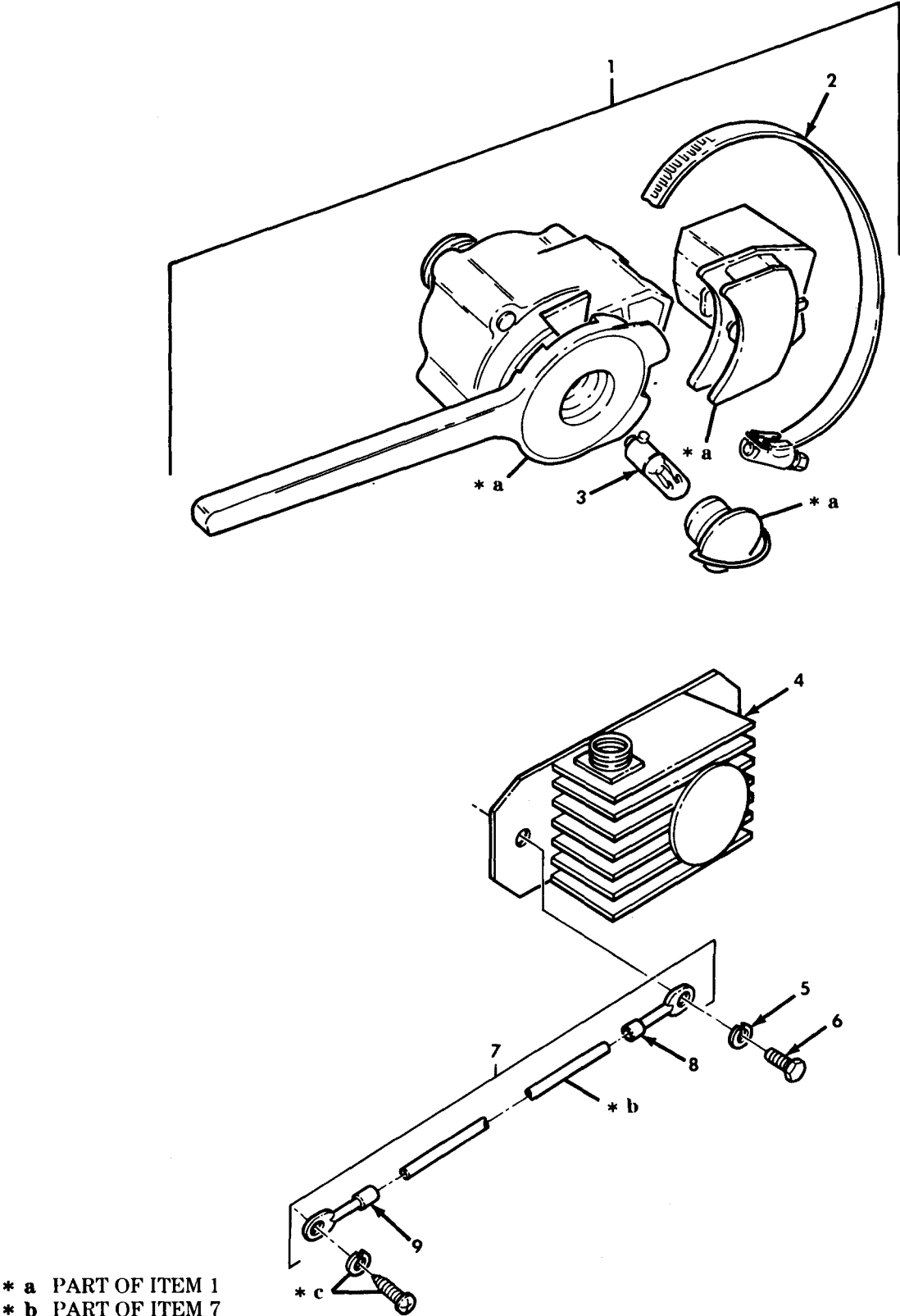
Figure 85. Control Unit and Directional Flasher
