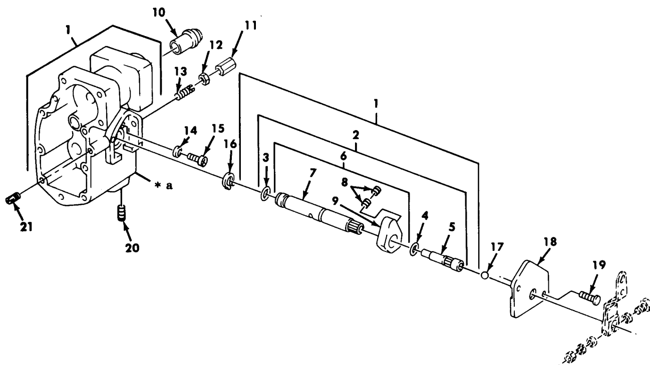
Figure 35. Fuel Pump Housing, VS.
