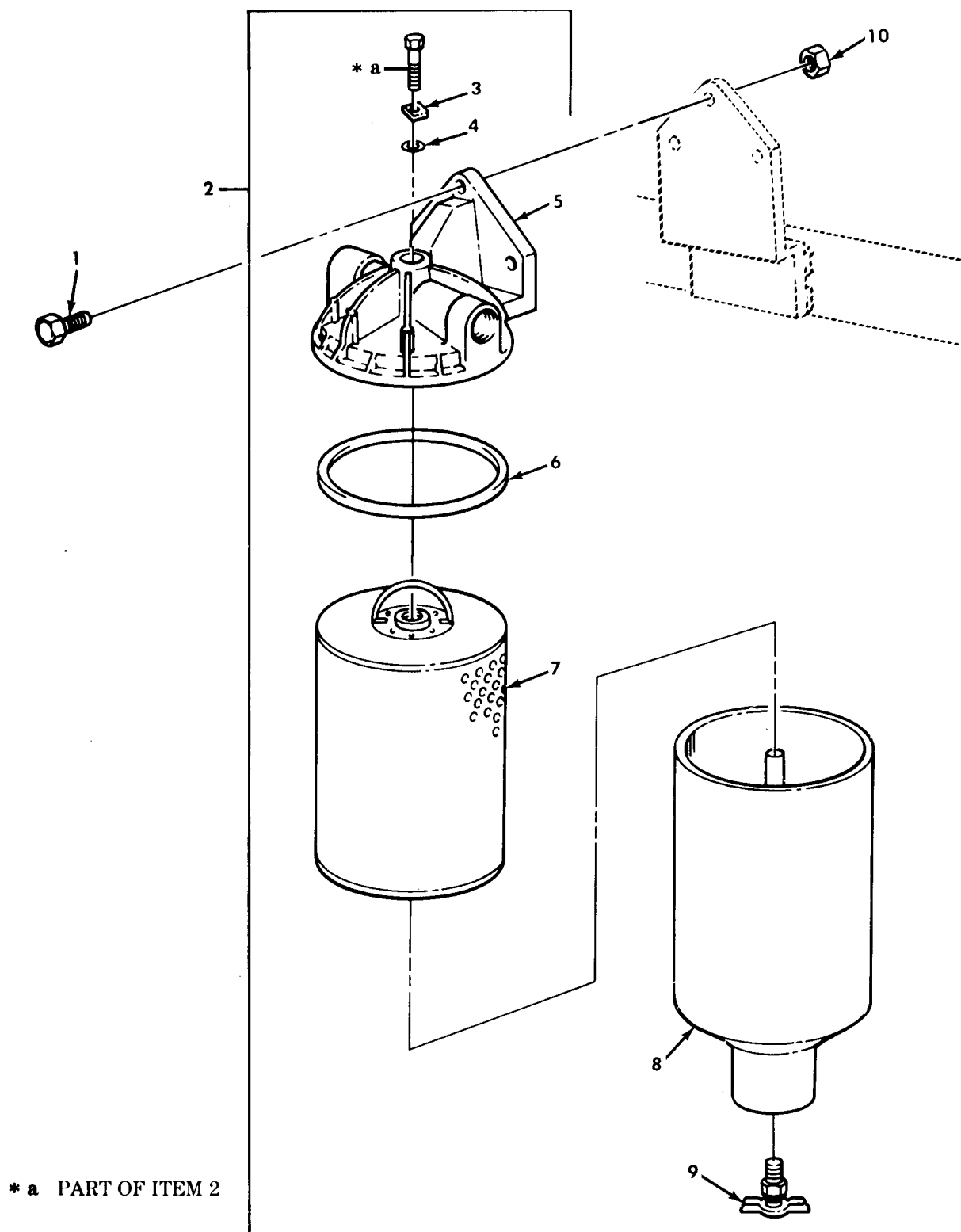
Figure 59. Fuel Filter, Water Separator, and Mounting Hardware.
