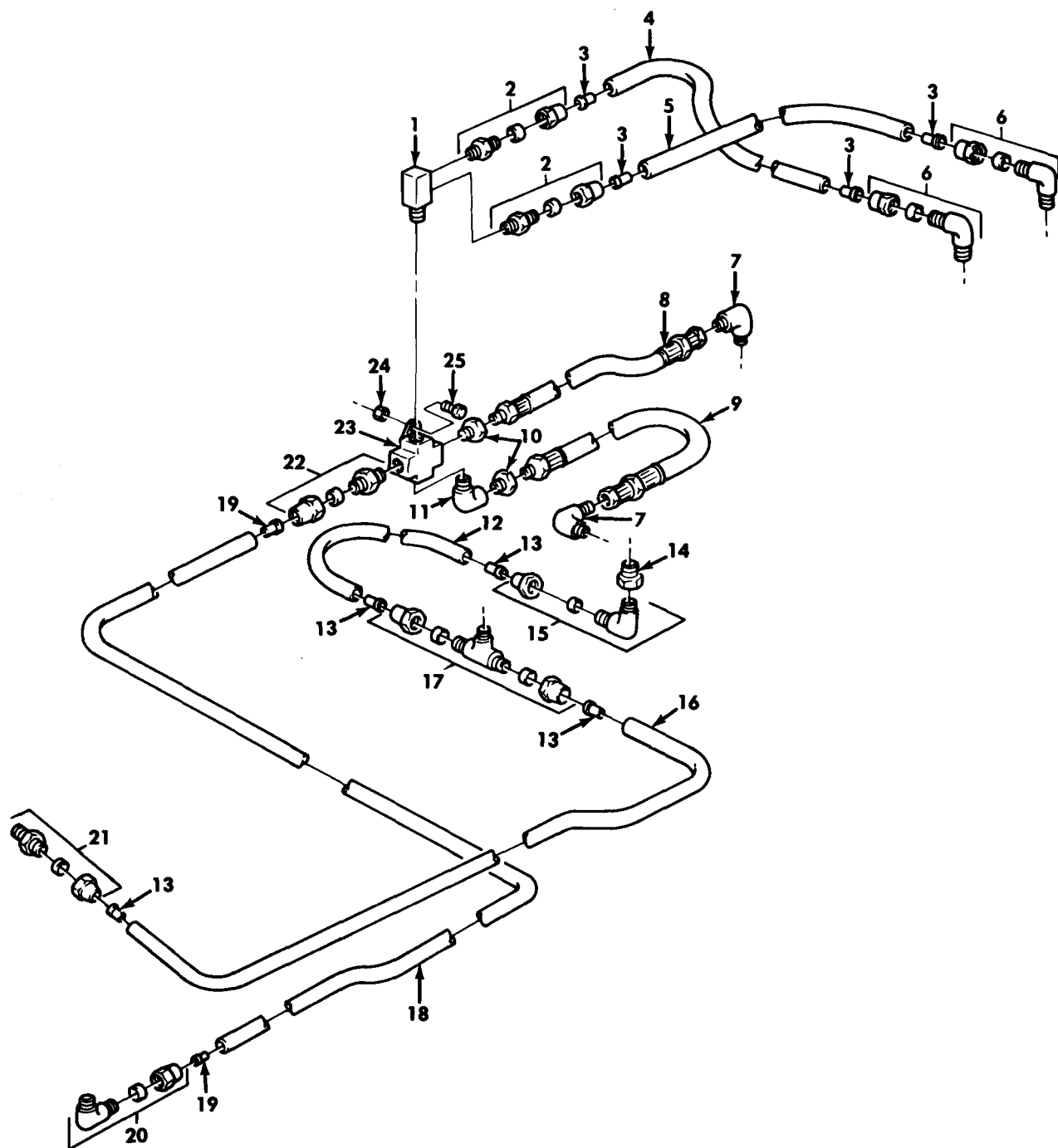
Figure 207. Vent Lines, Air Intake Manifold to Primary and Secondary Relay Valves and Rear Axle Vent Lines.
