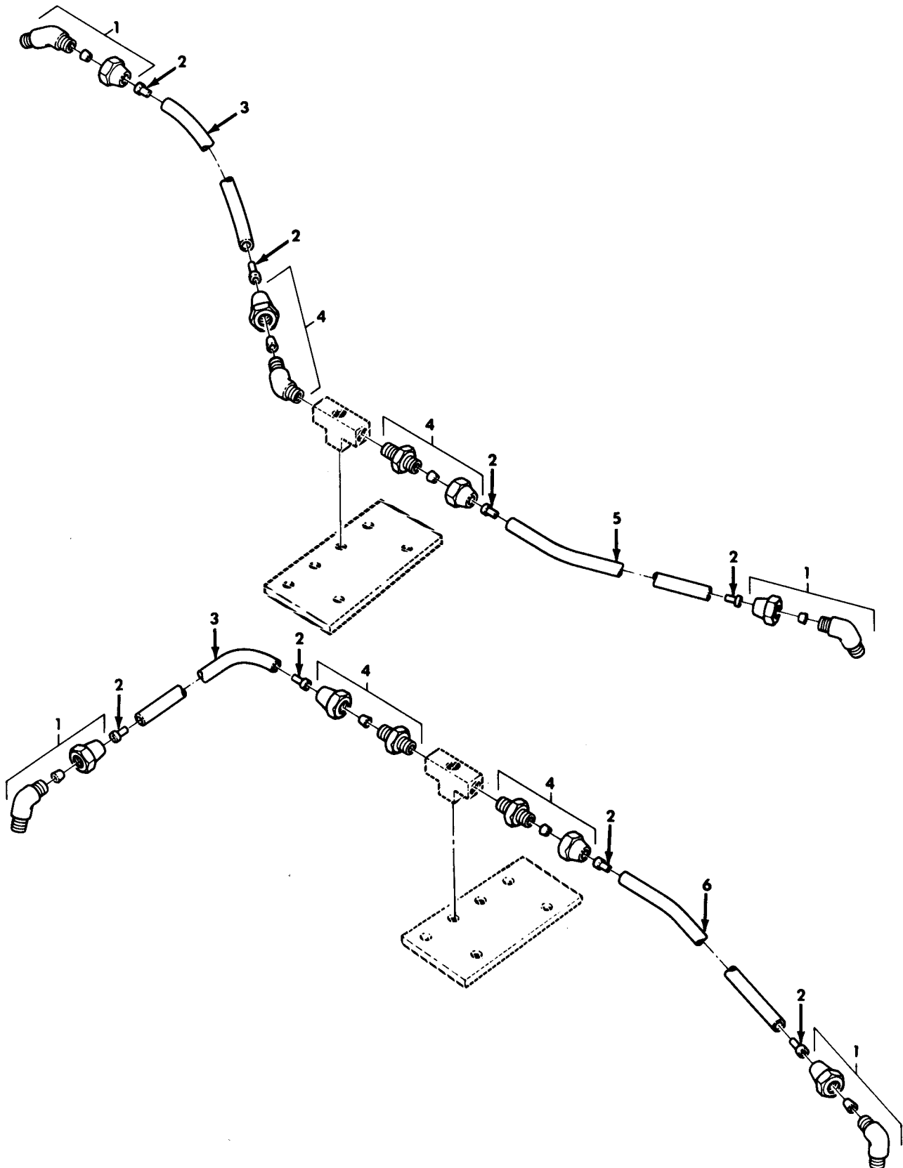
Figure 202. Failsafe Air Brake Chamber Lines.
