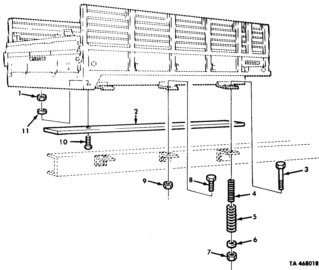
Figure 297. Standard Cargo, Dropside Cargo, and Mounting Hardware.
