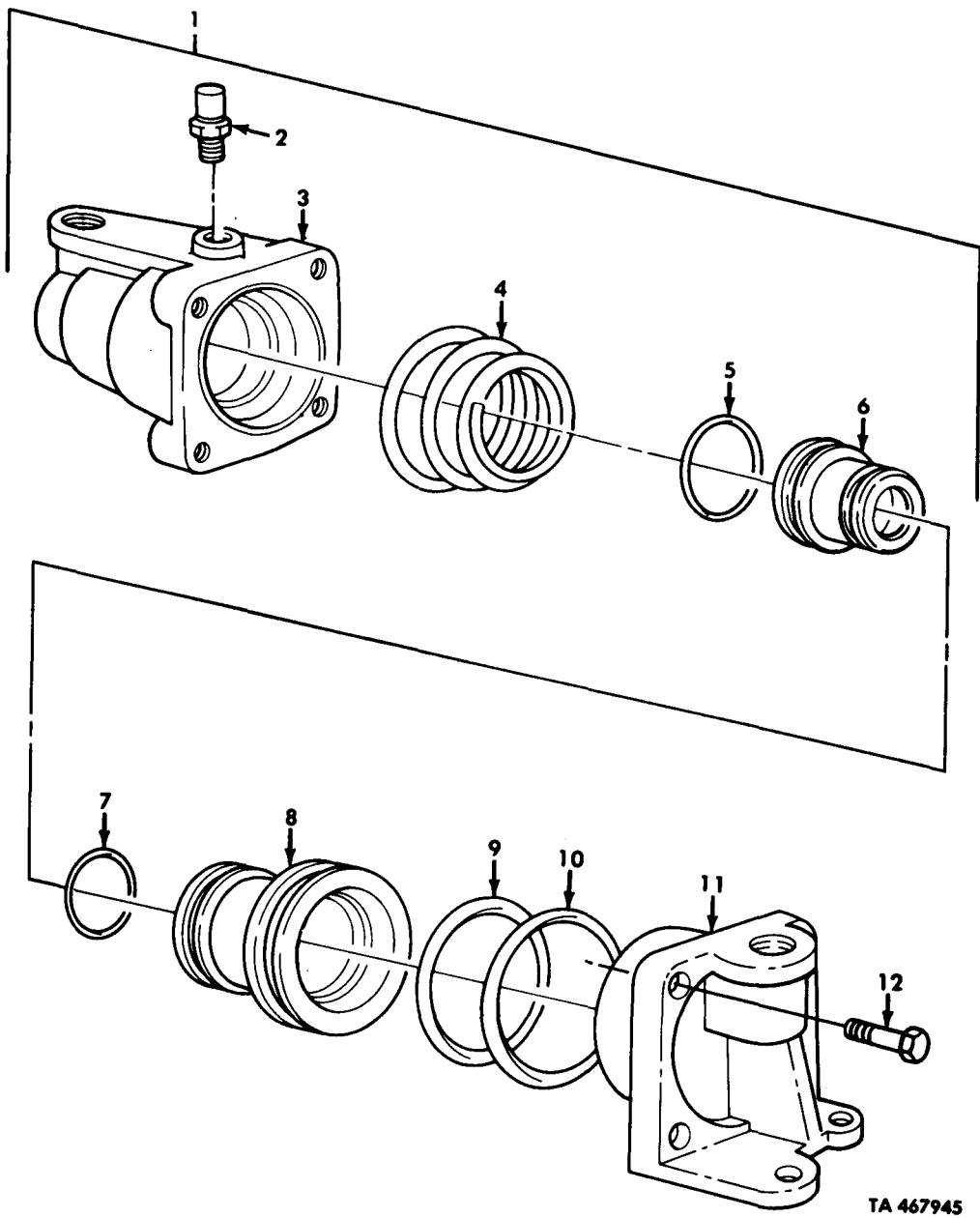
Figure 214. Front Air Brake Chamber Valve Assembly.
